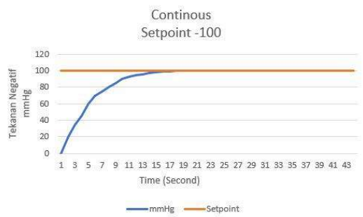
Gambar 4.7 Grafik mode continuous setpoint -100
