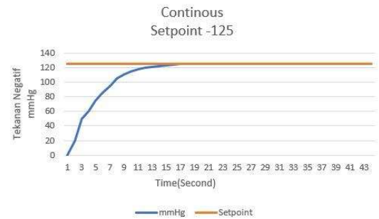
Gambar 4.8 Grafik mode continuous setpoint -125
