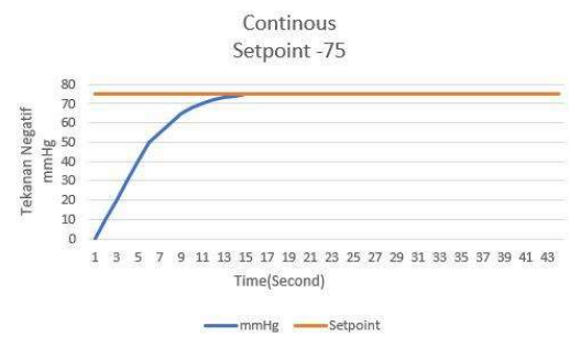
Gambar 4.6 Grafik mode continuous setpoint -75
