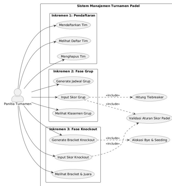
Gambar 2. Usecase Diagram
