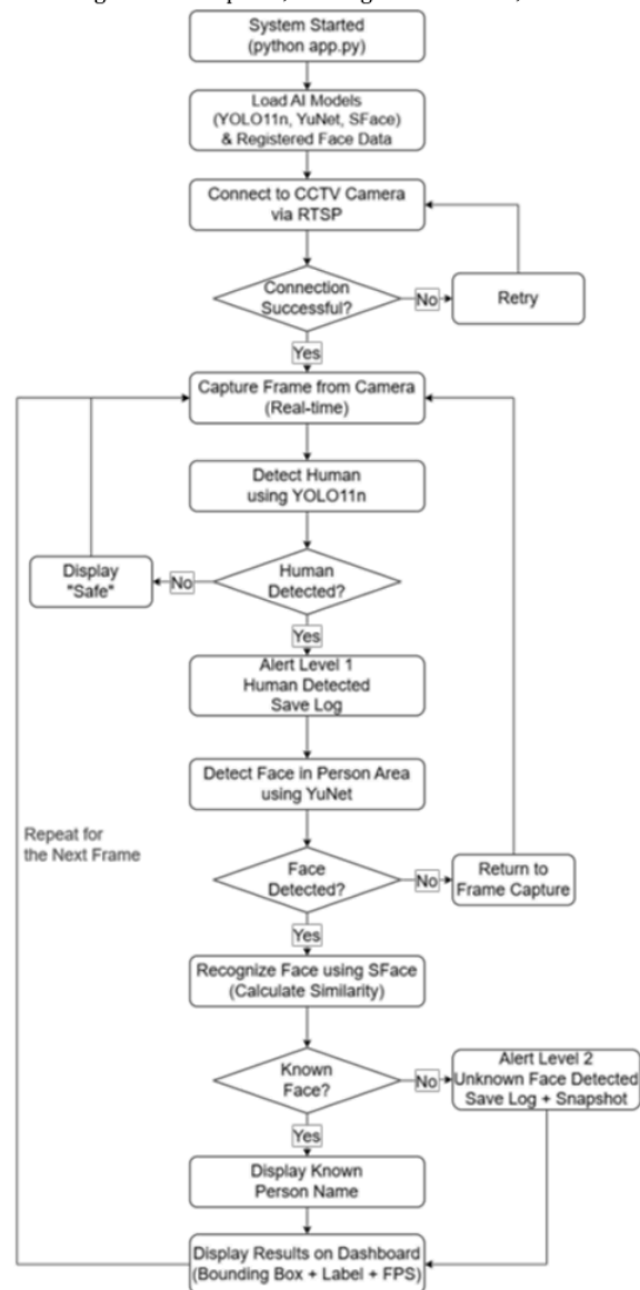
Figure 1. Flowchart System
