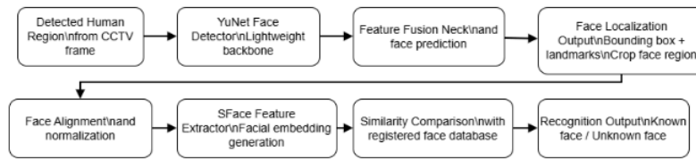
Figure 3. Face recognition architecture using YuNet and Sface
