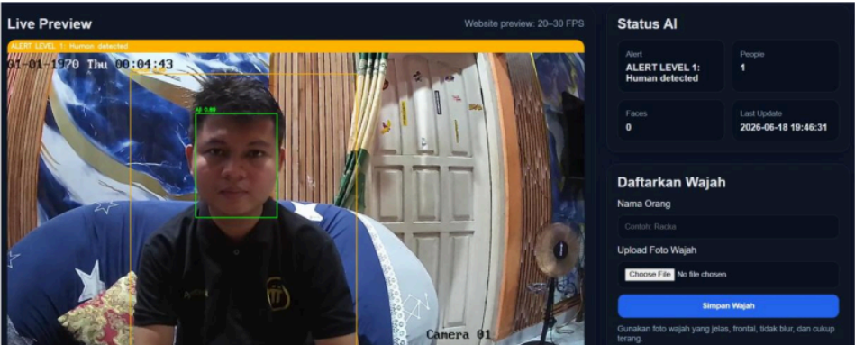
Figure 7. Example of registered face recognition testing
