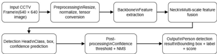
Figure 2. YOLO11n architecture for human detection
