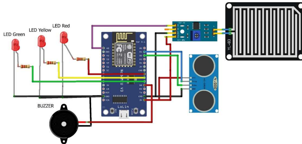
Gambar 1. Desain Hardware
