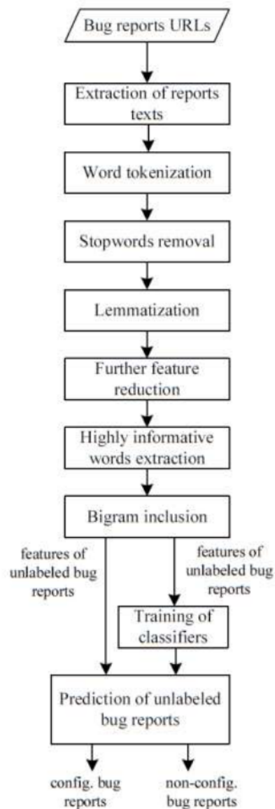
Figure 3. The Error Summary method process.
