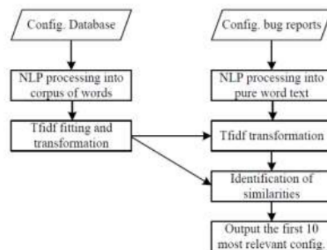
Figure 4. Identification of the Composition Error Summary.
