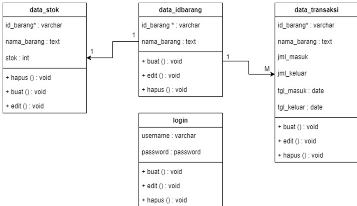
Gambar 1.2. Class Diagram
