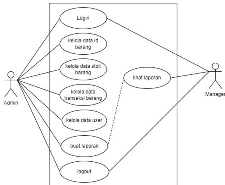
Gambar 1.1. Use Case Diagram
